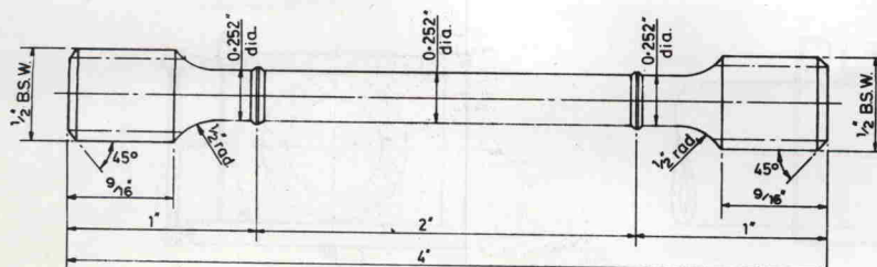
Figure 5. Tension specimen.
