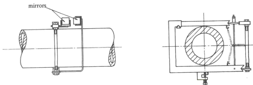
Figure 3. General arrangement of extensometer.
