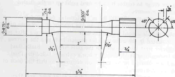
Figure 4. Torsion specimen.
